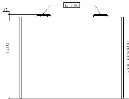
Over Cell Dimension
