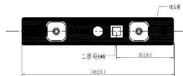
Dimension of Cover Plate
