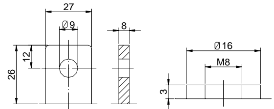
Terminal T20
